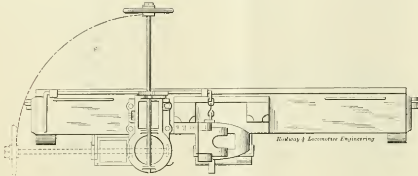
IMPROVED HAND BRAKE FOR FLAT CARS.
